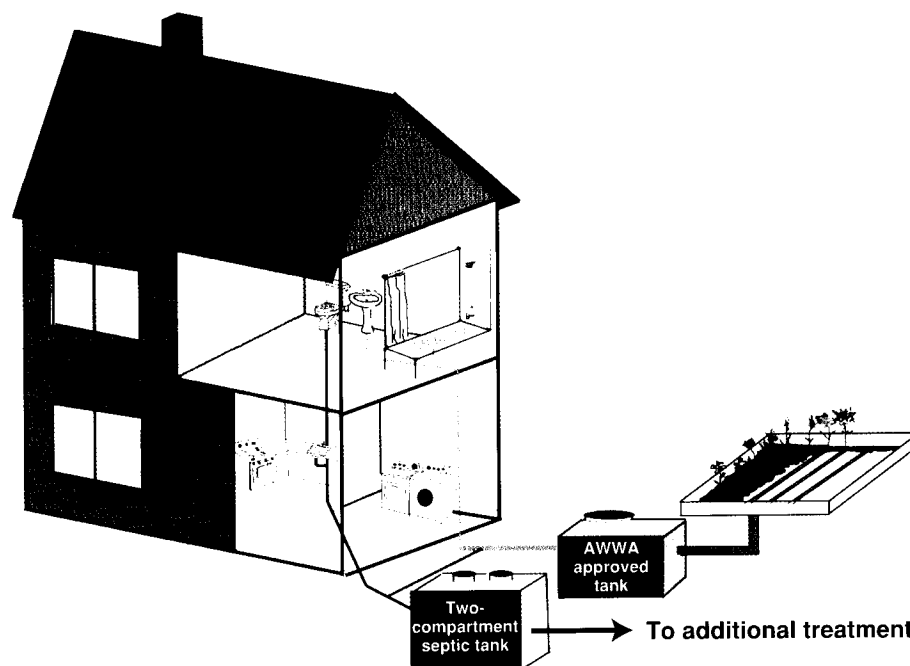
Figure 2. House diagram of separate blackwater and graywater plumbing systems.
