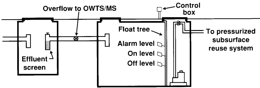
Figure 7. Settling tank and pump tank for pressurized graywater distribution.
